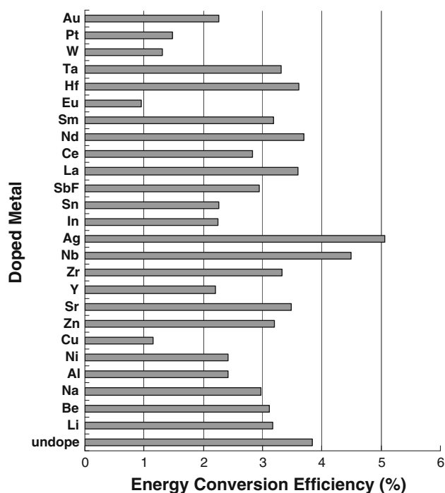
Fig. 3 Conversion efficiency of DSCs with various metal-doped \text{TiO}_2 electrodes
